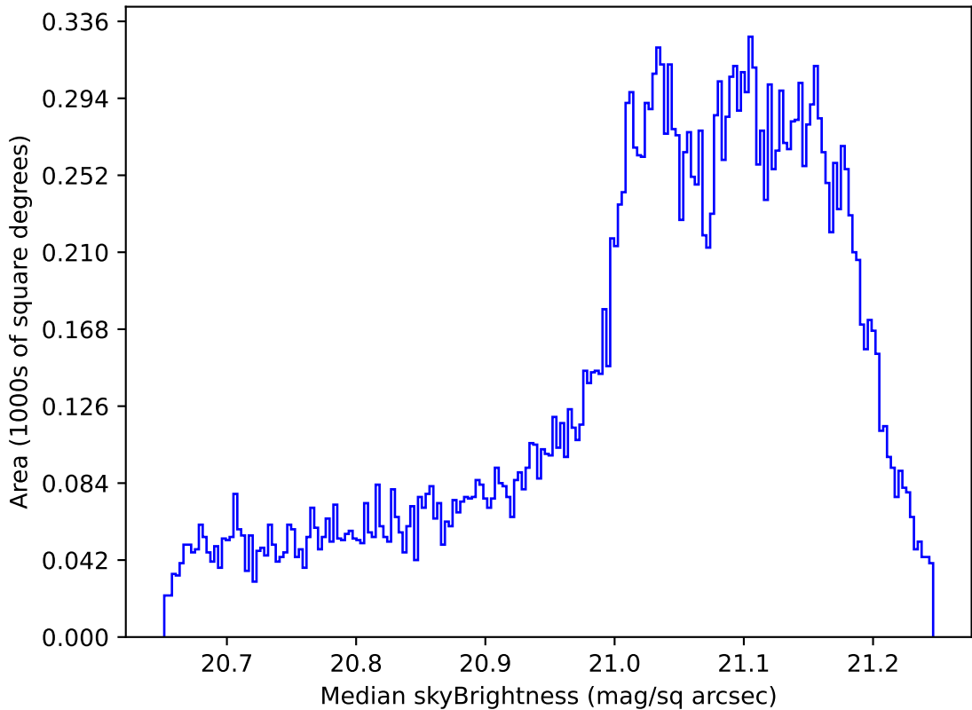
weather_cloudso35v3.4_10yrs All sky r band: Median skyBrightness
