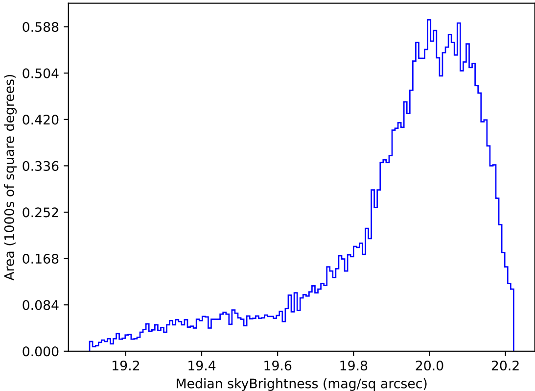
weather_cloudso35v3.4_10yrs All sky i band: Median skyBrightness
