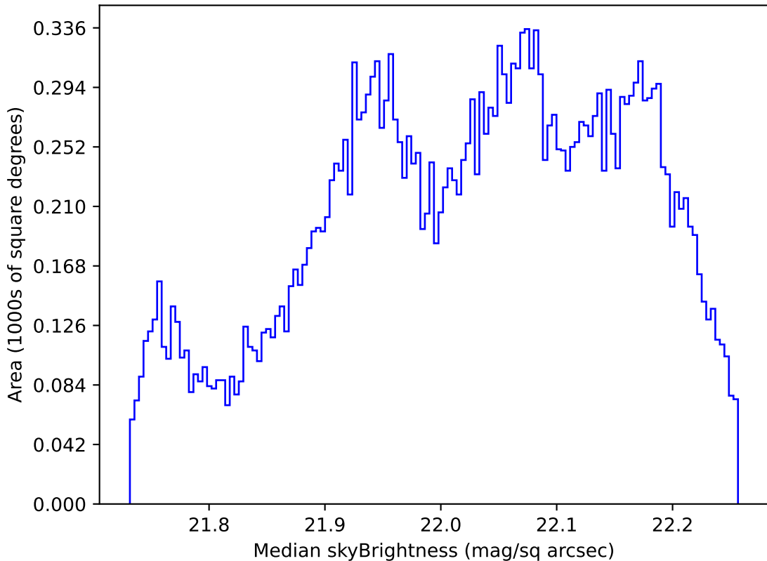
weather_cloudso35v3.4_10yrs All sky g band: Median skyBrightness
