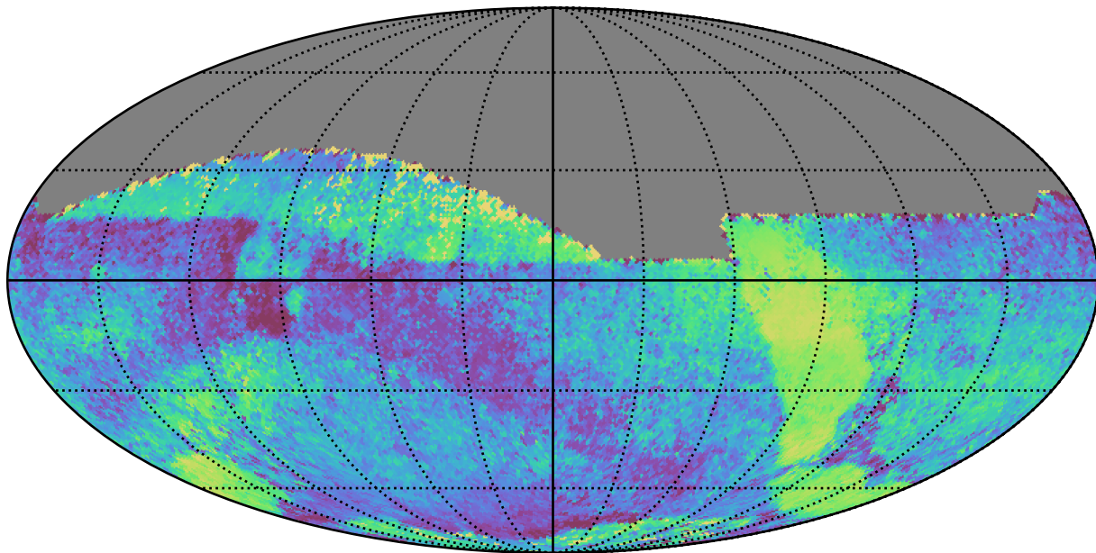
weather_cloudso35v3.4_10yrs All sky all bands: Median skyBrightness
