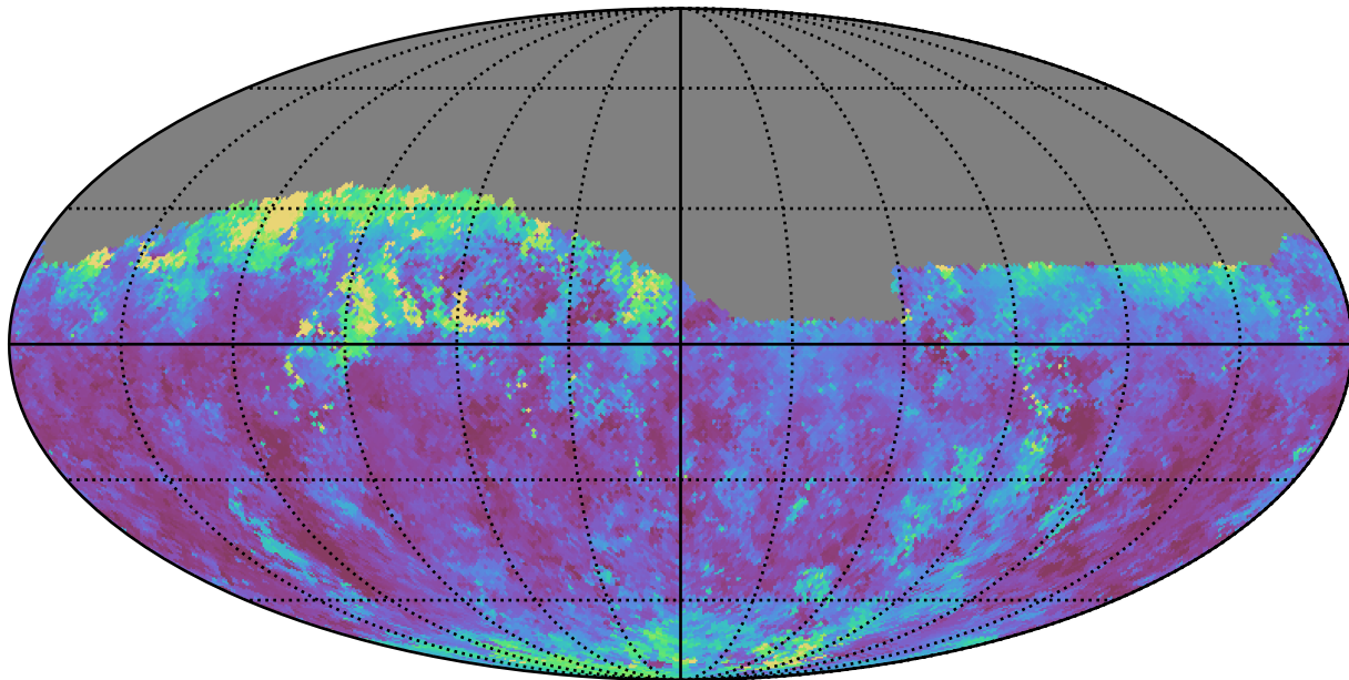
weather_cloudso35v3.4_10yrs Yr 1 z band: Median seeingGeom
