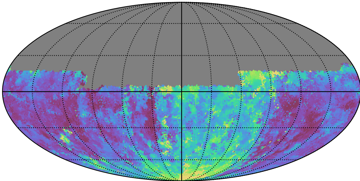
weather_cloudso35v3.4_10yrs Yr 1 u band: Median seeingGeom
