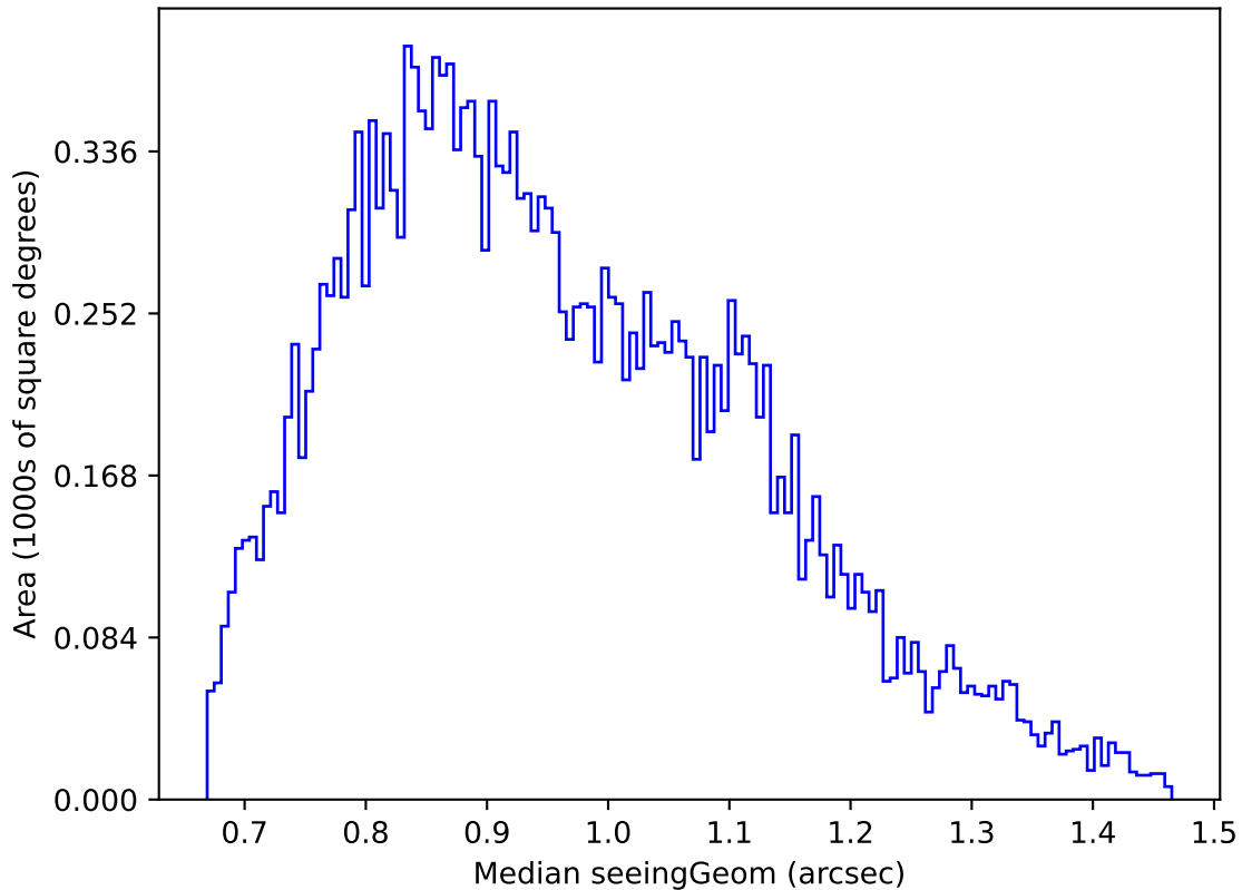
weather_cloudso35v3.4_10yrs Yr 1 u band: Median seeingGeom
