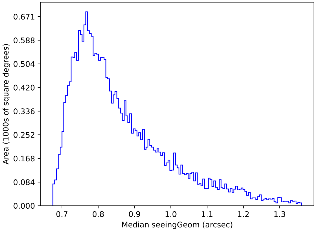
weather_cloudso35v3.4_10yrs Yr 1 r band: Median seeingGeom
