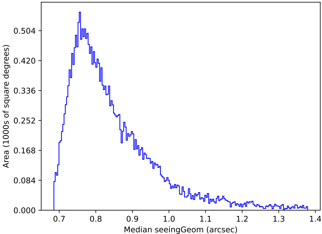
weather_cloudso35v3.4_10yrs Yr 1 i band: Median seeingGeom
