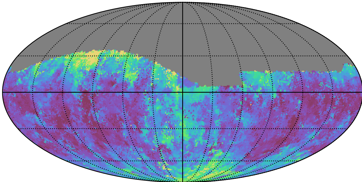
weather_cloudso35v3.4_10yrs Yr 1 g band: Median seeingGeom
