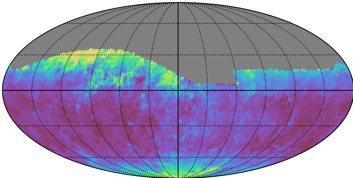
weather_cloudso35v3.4_10yrs Yr 1 all bands: Median seeingGeom
