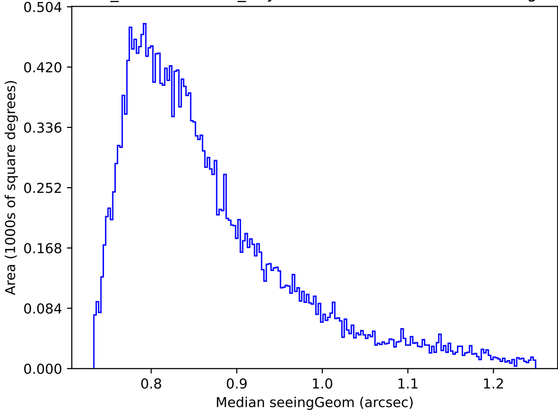
weather_cloudso35v3.4_10yrs Yr 1 all bands: Median seeingGeom
