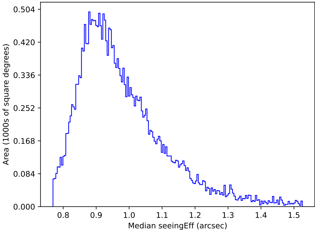
weather_cloudso35v3.4_10yrs Yr 1 z band: Median seeingEff
