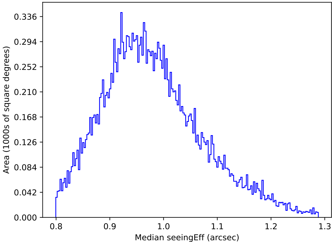
weather_cloudso35v3.4_10yrs Yr 1 y band: Median seeingEff
