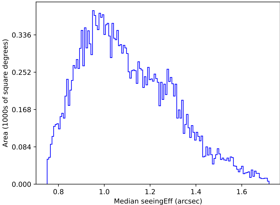
weather_cloudso35v3.4_10yrs Yr 1 u band: Median seeingEff
