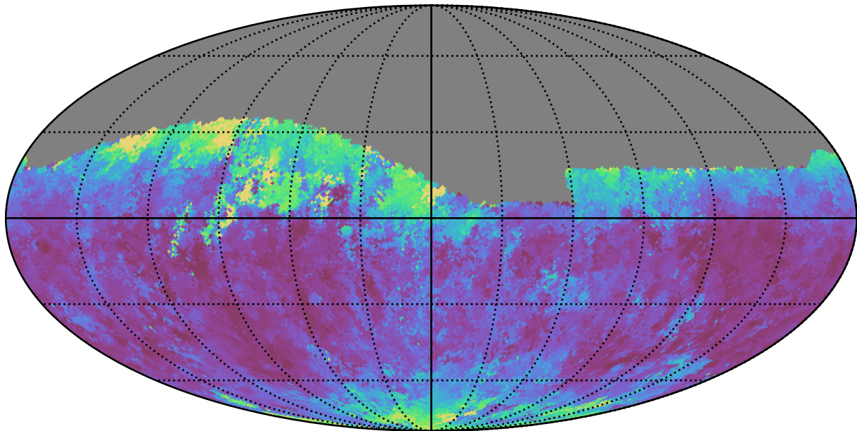
weather_cloudso35v3.4_10yrs Yr 1 r band: Median seeingEff
