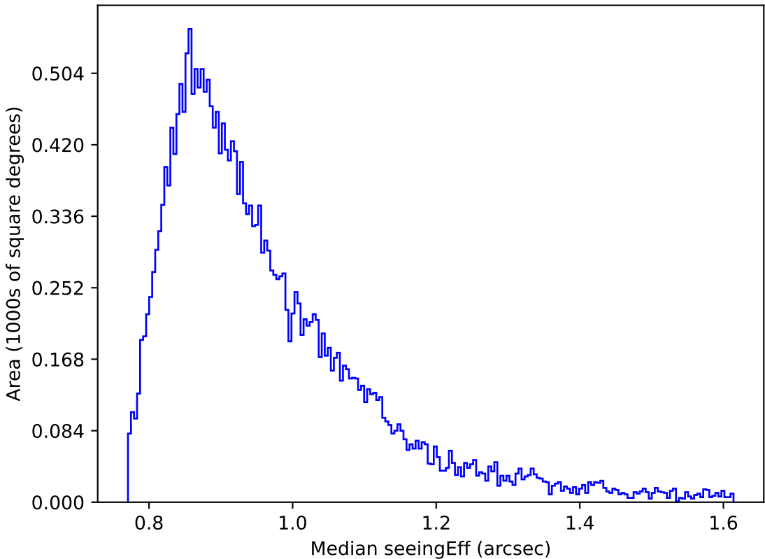
weather_cloudso35v3.4_10yrs Yr 1 i band: Median seeingEff
