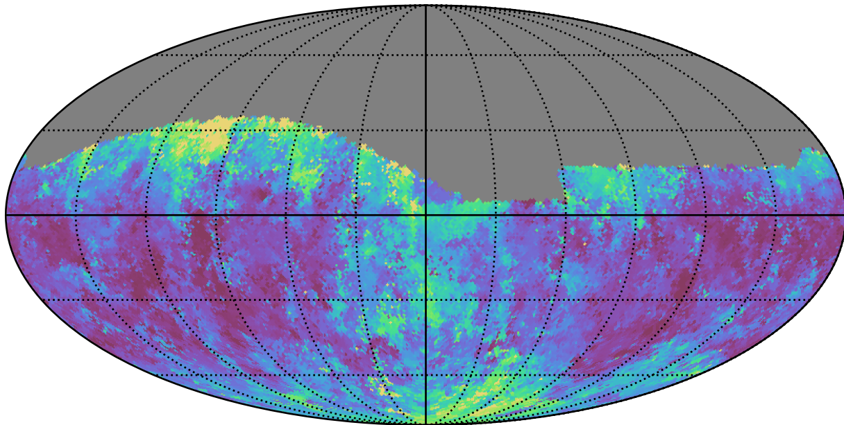
weather_cloudso35v3.4_10yrs Yr 1 g band: Median seeingEff
