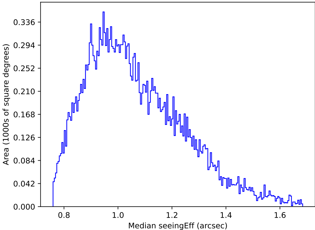
weather_cloudso35v3.4_10yrs Yr 1 g band: Median seeingEff
