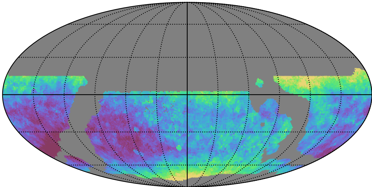
weather_cloudso35v3.4_10yrs WFD z band: Median seeingEff
