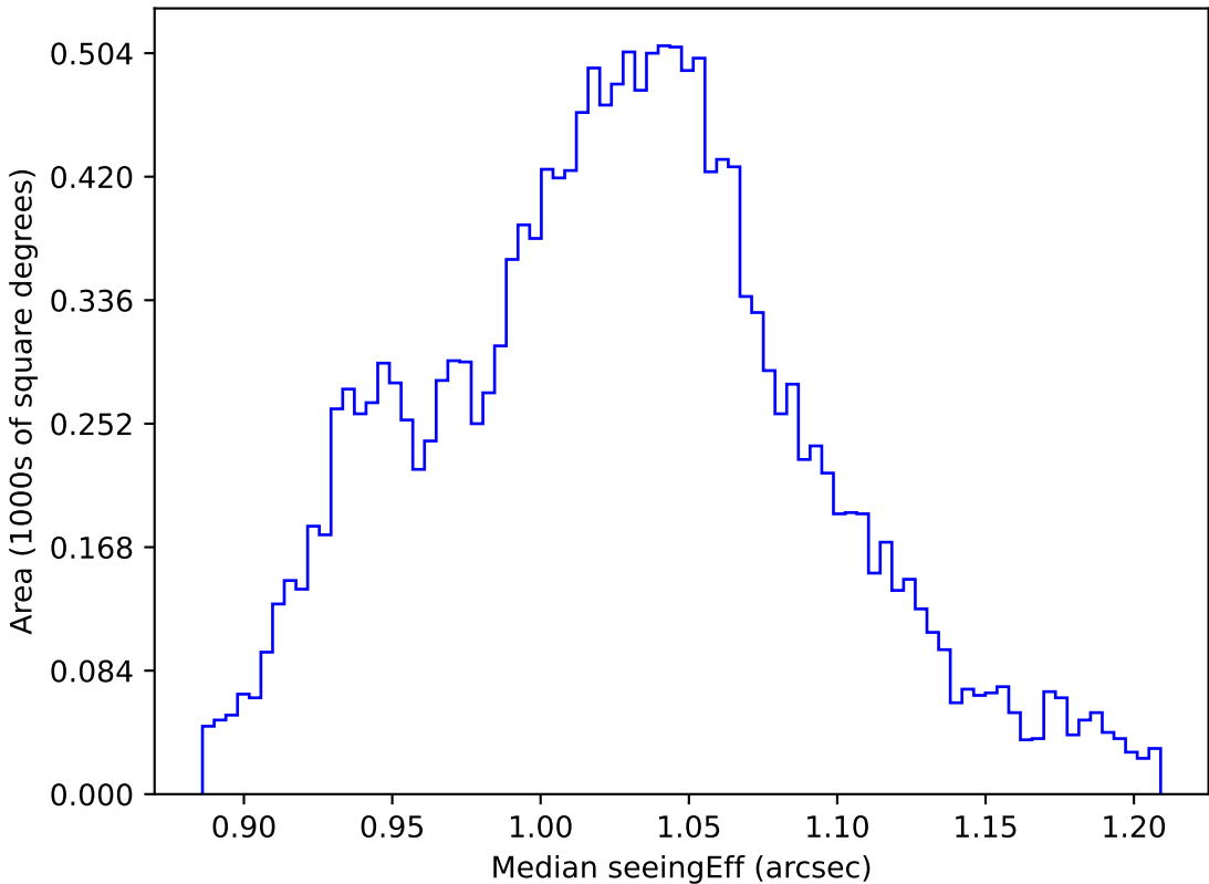
weather_cloudso35v3.4_10yrs WFD z band: Median seeingEff
