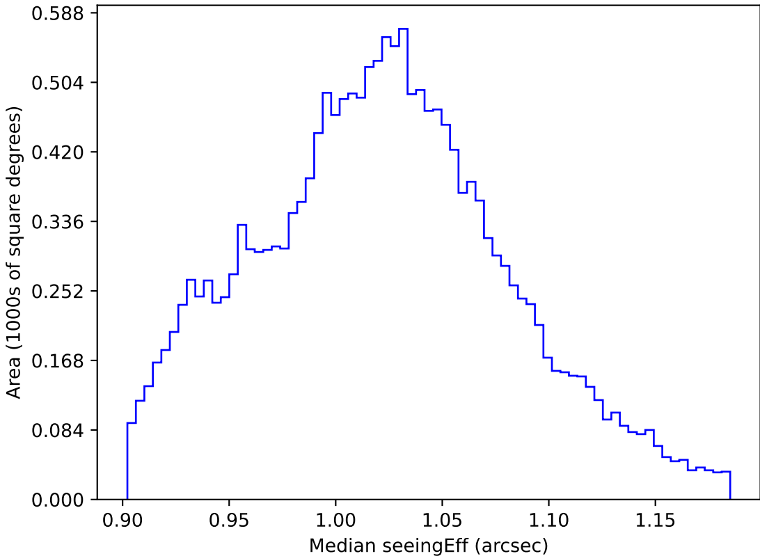
weather_cloudso35v3.4_10yrs WFD y band: Median seeingEff
