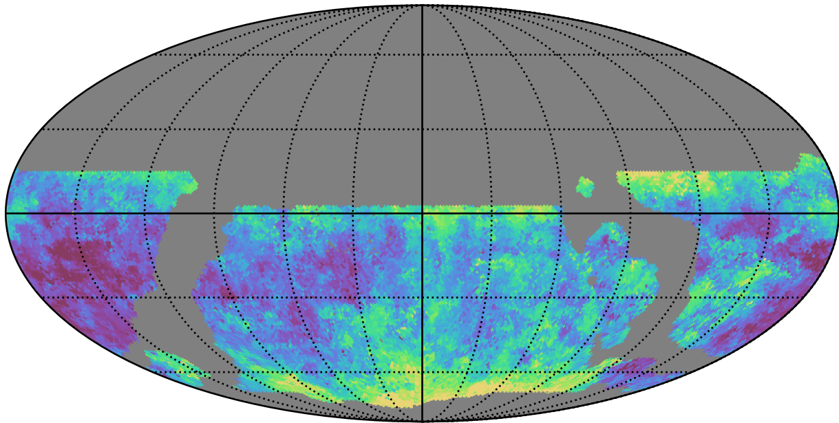
weather_cloudso35v3.4_10yrs WFD u band: Median seeingEff
