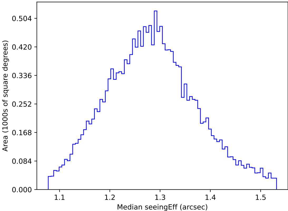
weather_cloudso35v3.4_10yrs WFD u band: Median seeingEff
