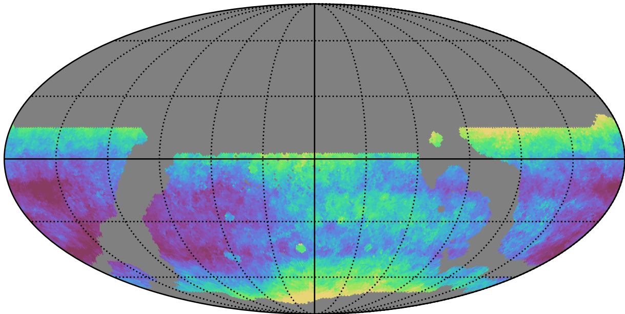
weather_cloudso35v3.4_10yrs WFD r band: Median seeingEff
