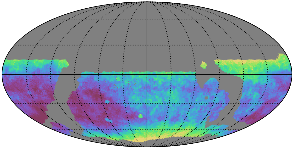
weather_cloudso35v3.4_10yrs WFD i band: Median seeingEff
