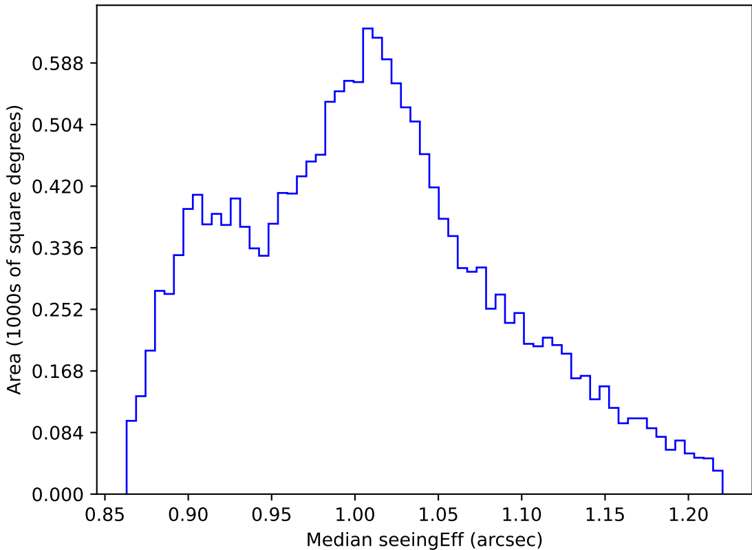
weather_cloudso35v3.4_10yrs WFD i band: Median seeingEff
