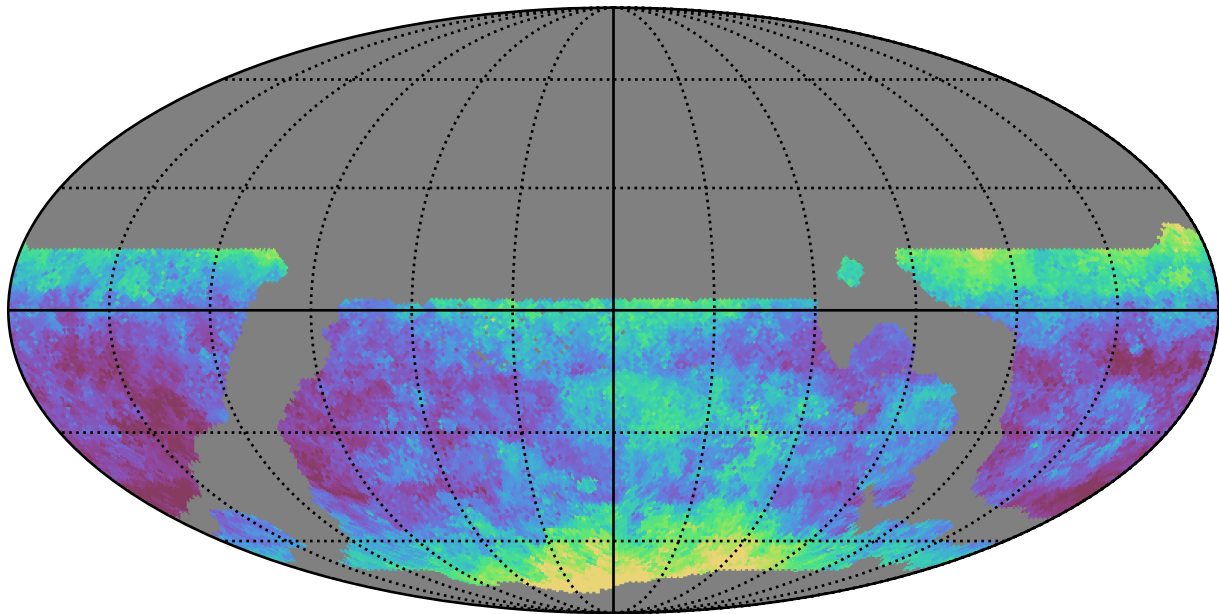
weather_cloudso35v3.4_10yrs WFD g band: Median seeingEff
