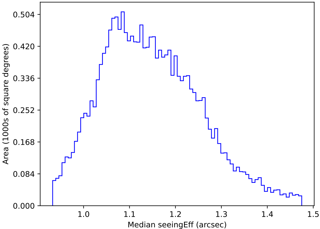
weather_cloudso35v3.4_10yrs WFD g band: Median seeingEff
