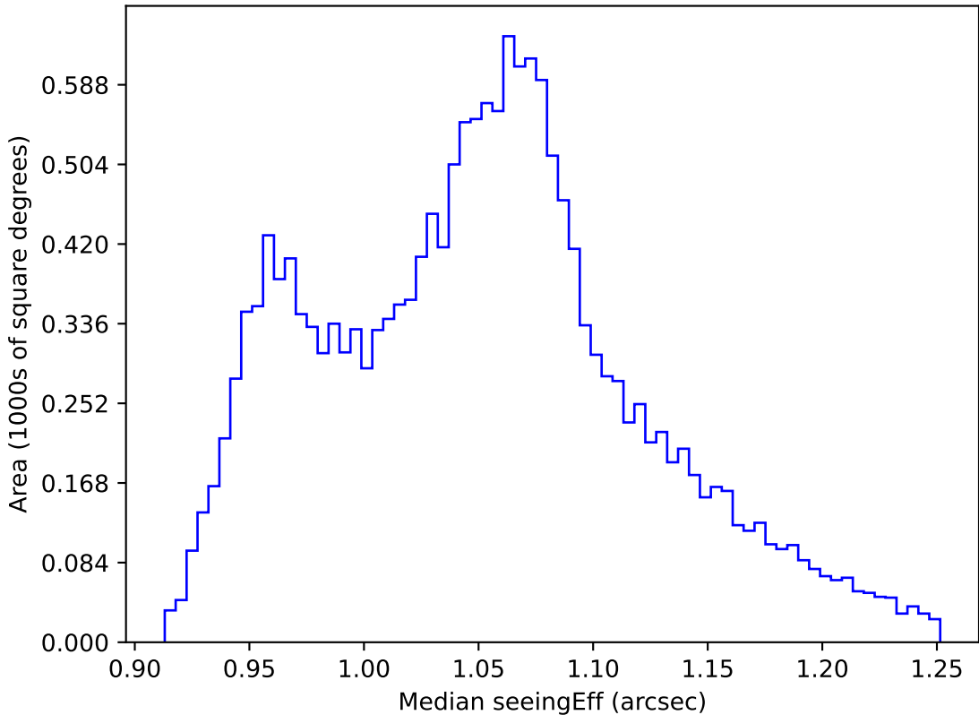
weather_cloudso35v3.4_10yrs WFD all bands: Median seeingEff
