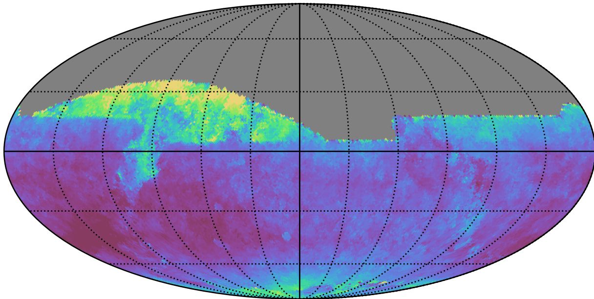
weather_cloudso35v3.4_10yrs All sky z band: Median seeingEff
