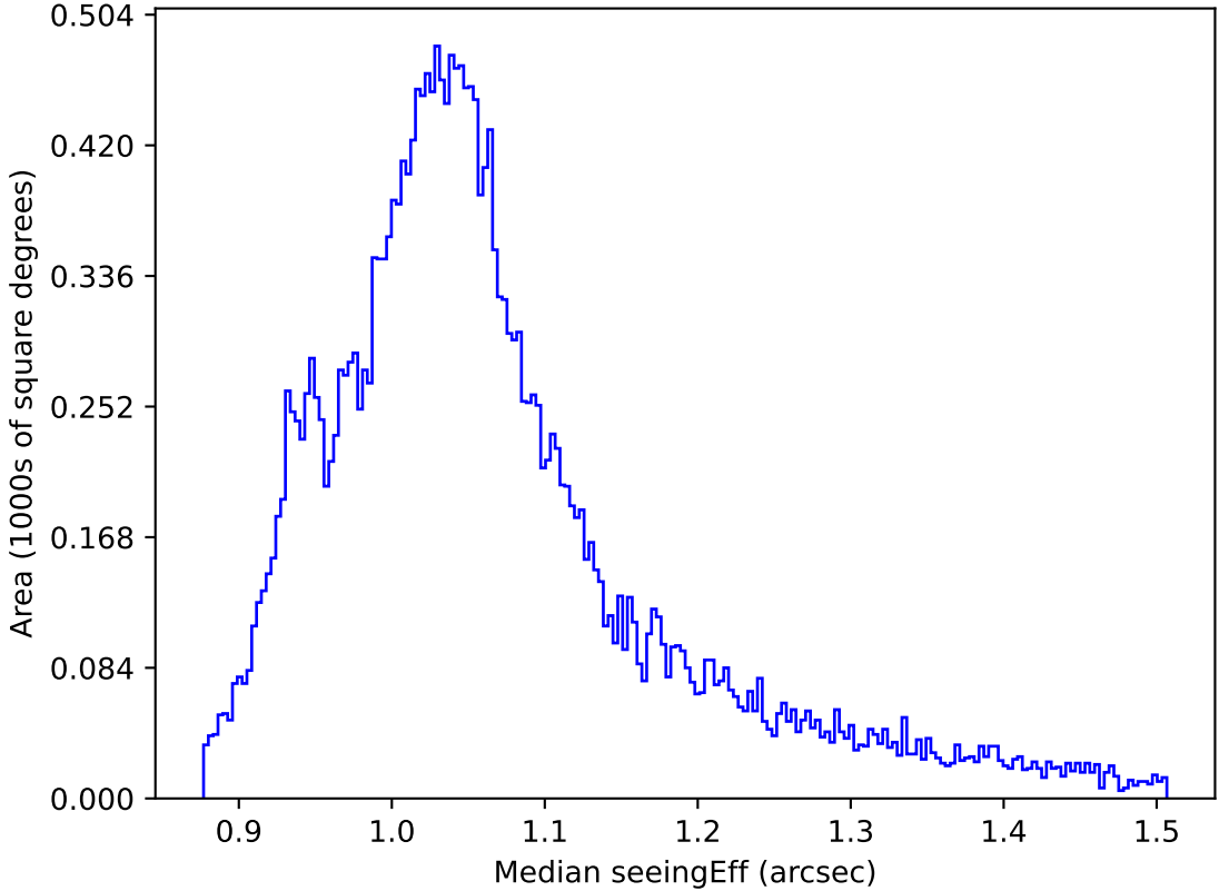
weather_cloudso35v3.4_10yrs All sky z band: Median seeingEff
