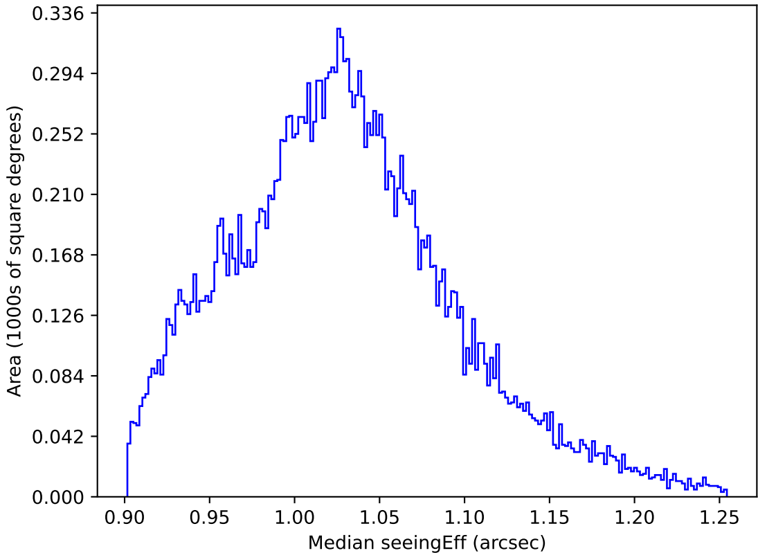
weather_cloudso35v3.4_10yrs All sky y band: Median seeingEff
