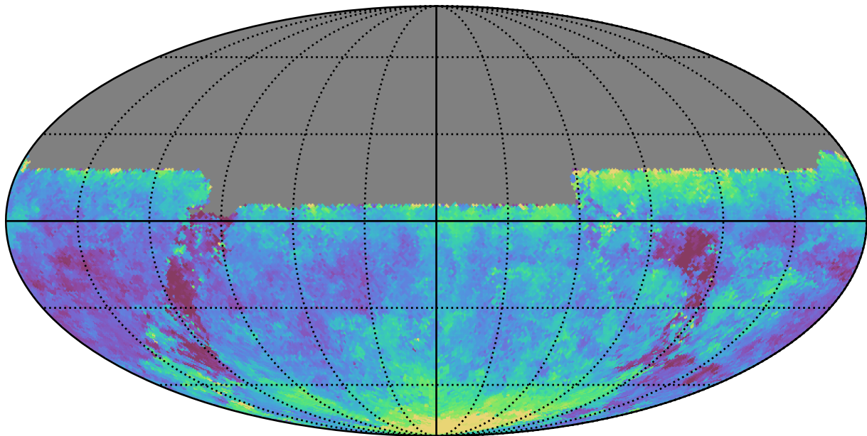
weather_cloudso35v3.4_10yrs All sky u band: Median seeingEff
