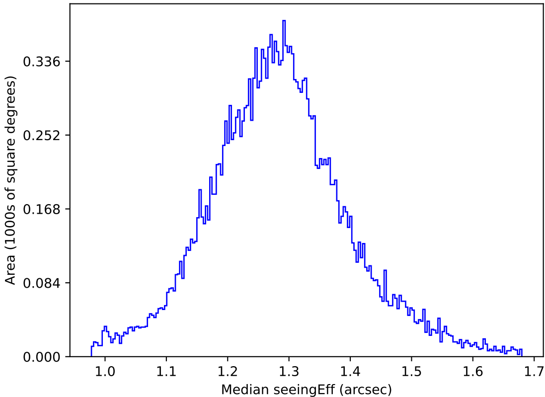
weather_cloudso35v3.4_10yrs All sky u band: Median seeingEff
