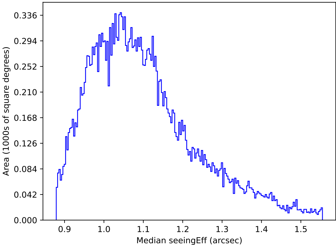
weather_cloudso35v3.4_10yrs All sky r band: Median seeingEff
