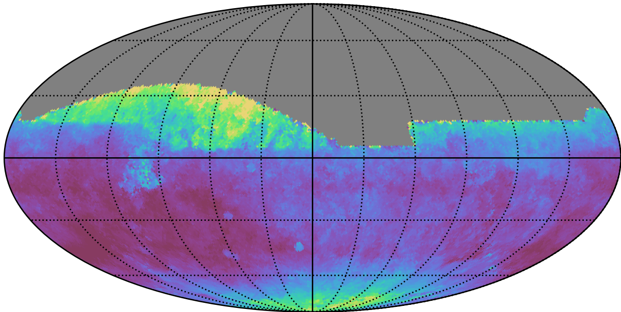
weather_cloudso35v3.4_10yrs All sky i band: Median seeingEff
