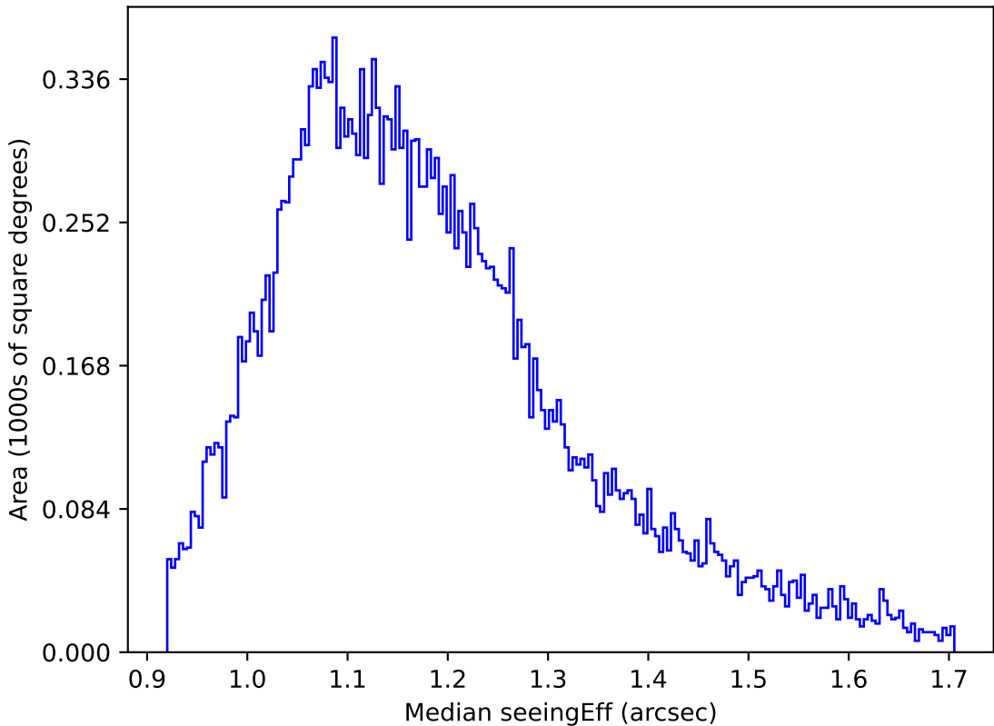
weather_cloudso35v3.4_10yrs All sky g band: Median seeingEff
