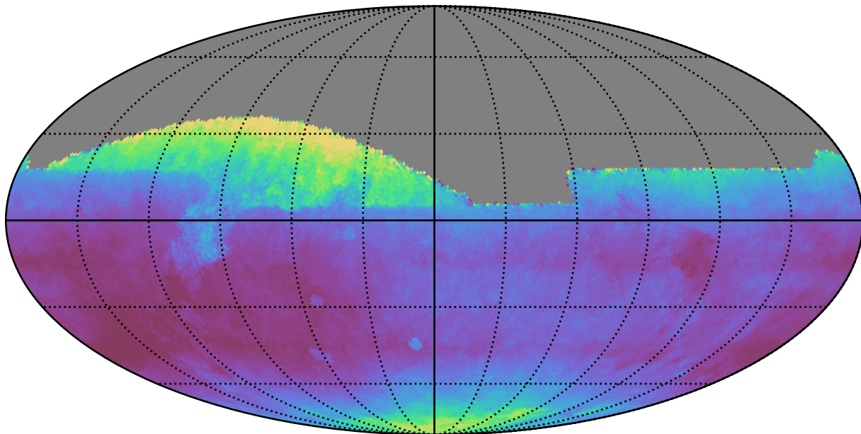
weather_cloudso35v3.4_10yrs All sky all bands: Median seeingEff
