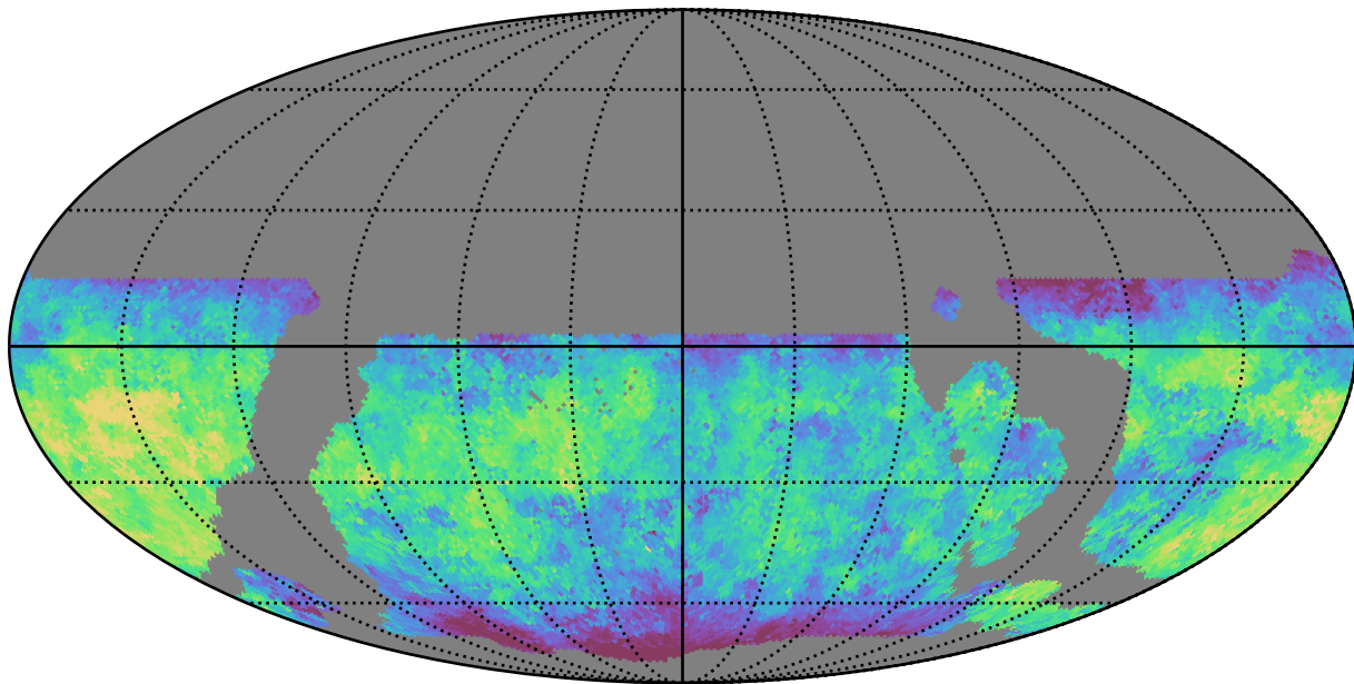
weather_cloudso35v3.4_10yrs WFD u band: Median saturation_mag
