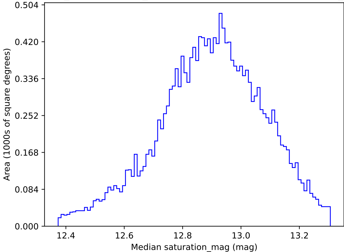
weather_cloudso35v3.4_10yrs WFD u band: Median saturation_mag
