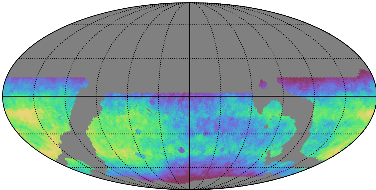
weather_cloudso35v3.4_10yrs WFD r band: Median saturation_mag
