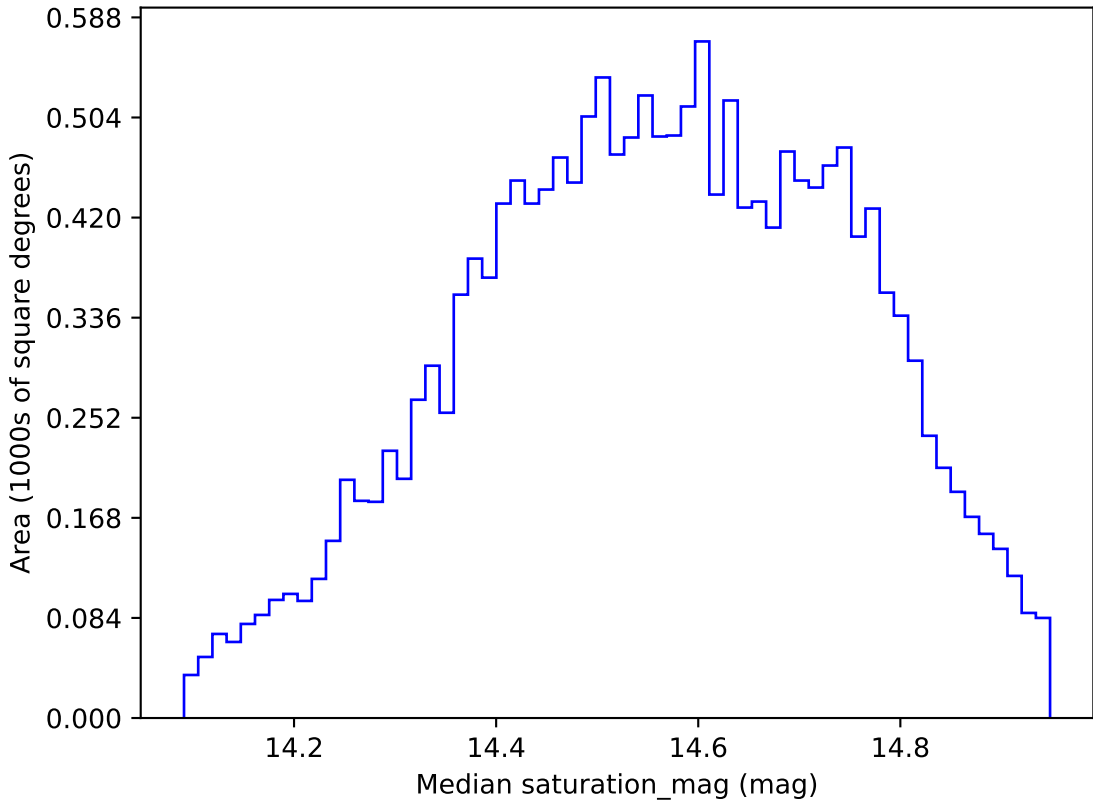
weather_cloudso35v3.4_10yrs WFD r band: Median saturation_mag
