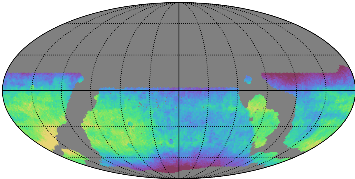
weather_cloudso35v3.4_10yrs WFD all bands: Median saturation_mag
