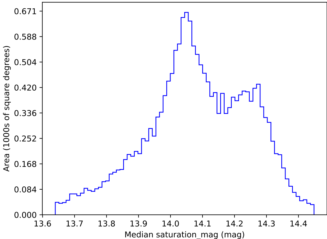
weather_cloudso35v3.4_10yrs WFD all bands: Median saturation_mag
