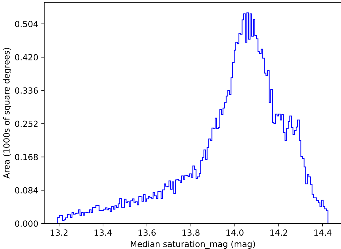
weather_cloudso35v3.4_10yrs All sky z band: Median saturation_mag
