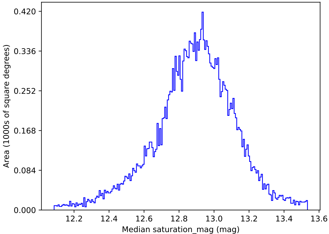
weather_cloudso35v3.4_10yrs All sky u band: Median saturation_mag
