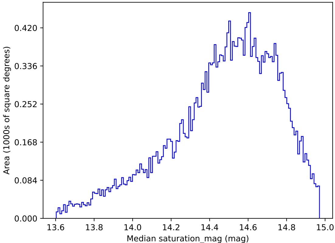
weather_cloudso35v3.4_10yrs All sky r band: Median saturation_mag
