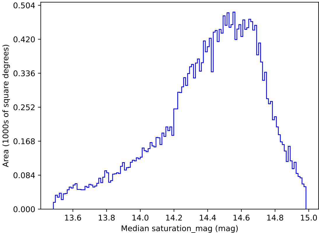
weather_cloudso35v3.4_10yrs All sky g band: Median saturation_mag
