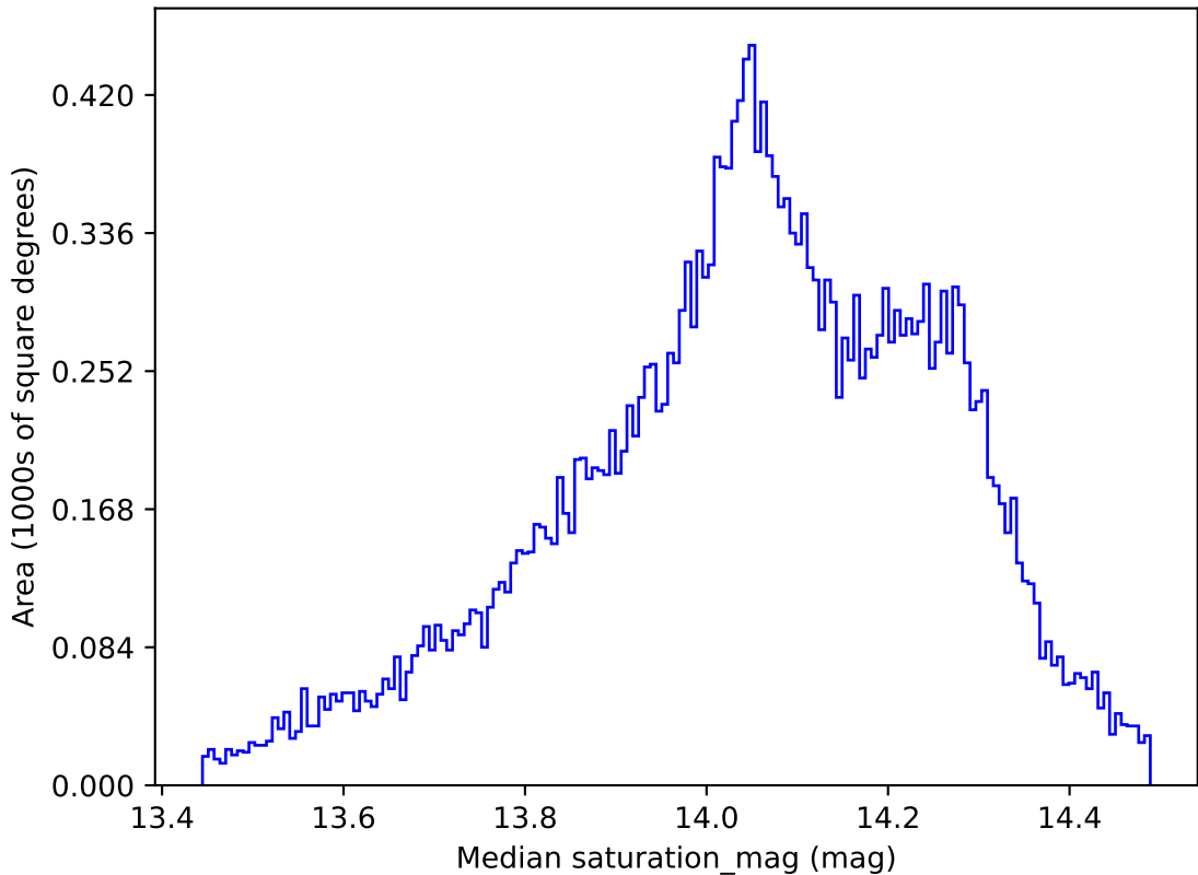
weather_cloudso35v3.4_10yrs All sky all bands: Median saturation_mag
